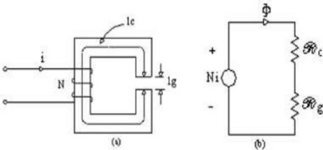
Figure 3. Magnetic nucleus with air gap (a) and an equivalent magnetic circuit (b).
